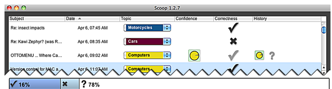
Fig. 9. (Top): The user tested three of the messages (the dark ✓ and ✗ marks), so they no longer show a priority. Then the computer inferred the third message to be correct (light gray ✓). Because the user’s last test caused the computer to infer new information, the History column shows the prior values of what changed. (These values move right with each new change, until they are pushed off the screen.) (Bottom): A test coverage bar informs users how many topic predictions have been judged (by the user or the computer) to be correct (✓) or incorrect (✗).
