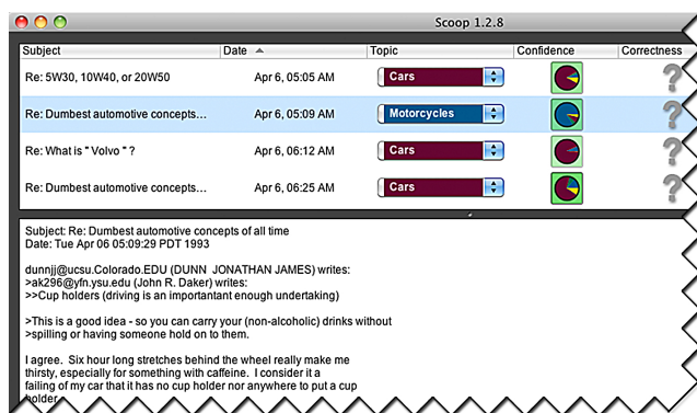
Fig. 1. A user interface to allow end users to test a classifier [32]. This classifier takes a message (input) and produces a topic label (output). The pie chart depicts the classifier’s confidence that the message belongs in the red category (Cars), the blue category (Motorcycles), etc. A user can mark any message’s topic label as right or wrong; these marked messages are the test cases.
