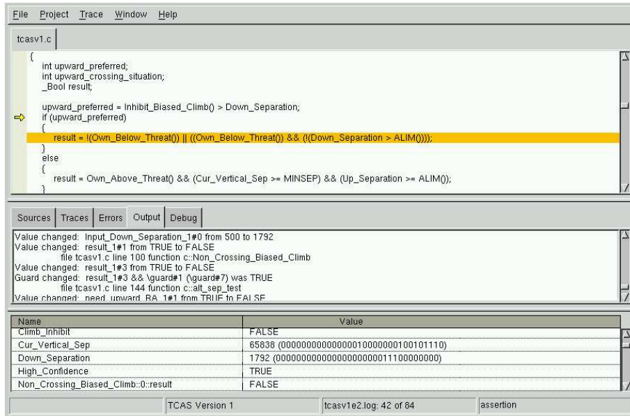
Fig. 1. Correctly locating the error in tcas.c .
